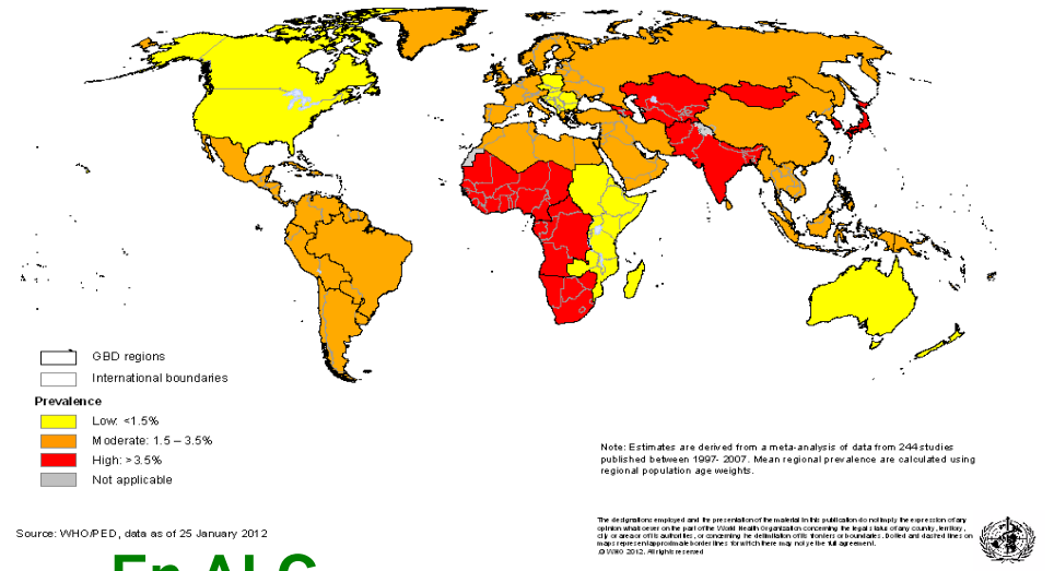
Anti-HCV seroprevalence by GBD region, 2005
