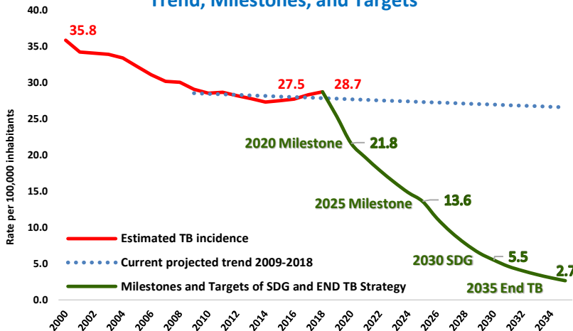
Estimated TB incidence in the Americas: Trend, Milestones, and Targets
