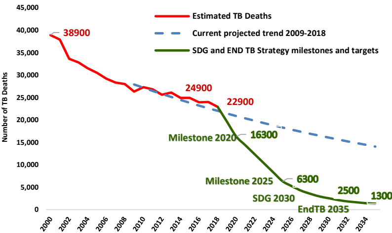
Estimated TB Deaths in the Americas: Trend, Milestones, and Targets
